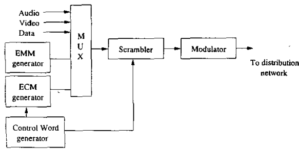
Fig. 2. Major components of the CA head-end architecture
