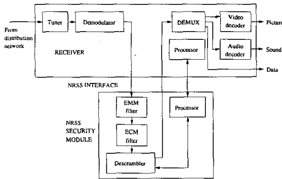
Fig. 3. NRSS security module and its host
