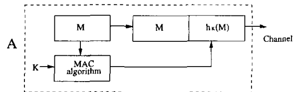
Fig. 5. Authentication with a MAC
