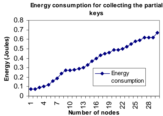
Figure 18. Energy consumption
