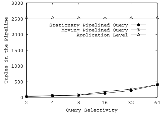
Figure 10: Pipelined operators with Join.
