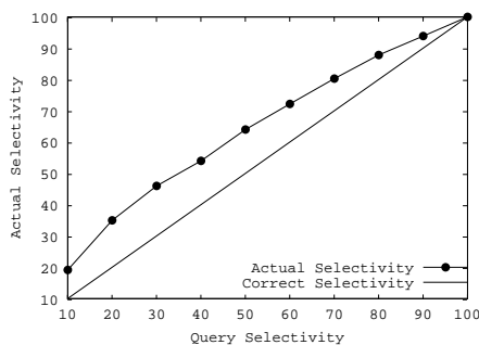
Figure 12: Query selectivity.
