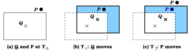
Figure 3: Uncertainty in moving queries.
