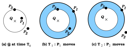
Figure 4: Uncertainty in static NN queries.
