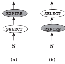
Figure 3: Partitioned sliding-window
